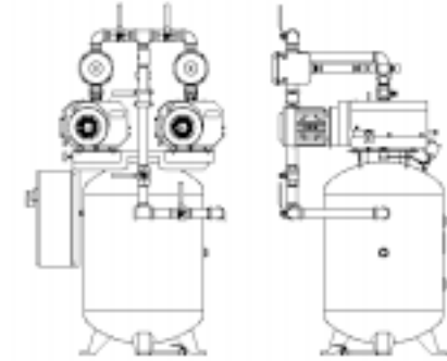
Vertical Tank Mounted Duplex
