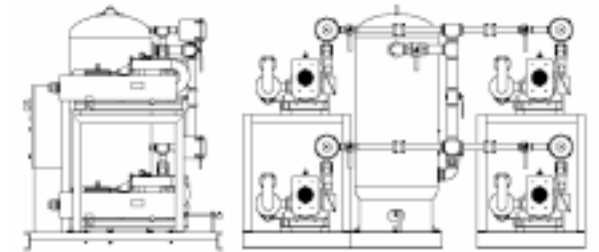
Stack Mounted Quadruplex
