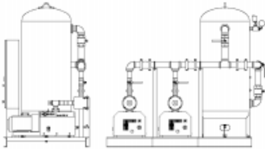
Base Mounted Duplex
