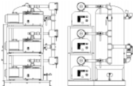
Stack Mounted Triplex
